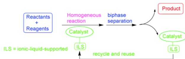
Fig. 2: Ionic liquids in organic synthesis
