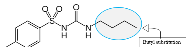
Fig. 6: Structure of tolbutamide (1950)/Carbutamide if NH 2 at Para position (1956)
