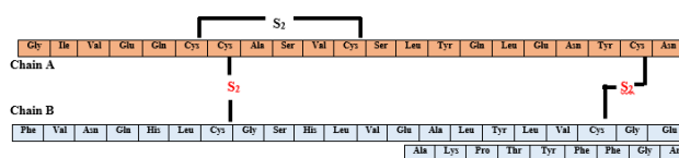
Fig. 5: Structure of insulin
