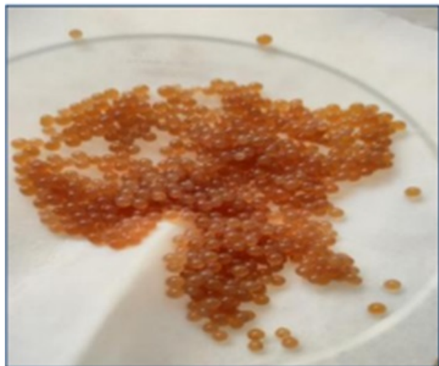
Figure 4: Tamarind microspheres
